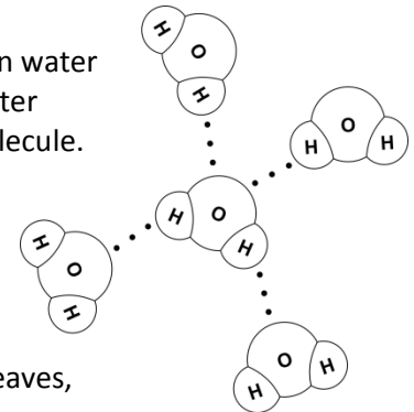
Figure 2: Hydrogen Bonding
