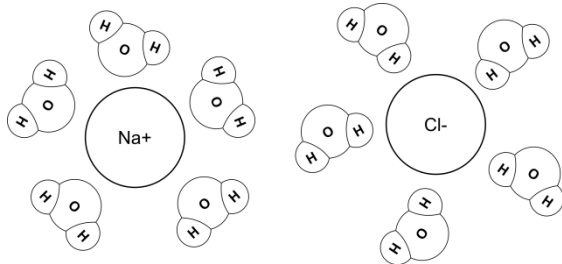
Figure 3: Hydration Spheres
